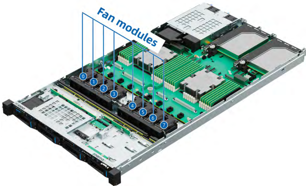
Figure 5-25 Fan Module Locations
