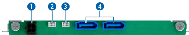
Figure 5-32 2 × M.2 Drive Backplane
