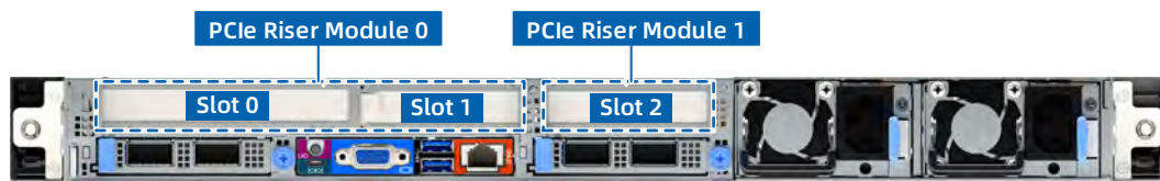
Figure 5-16 PCIe Slots
