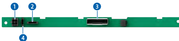
Figure 5-33 2 × E1.S Drive Backplane
