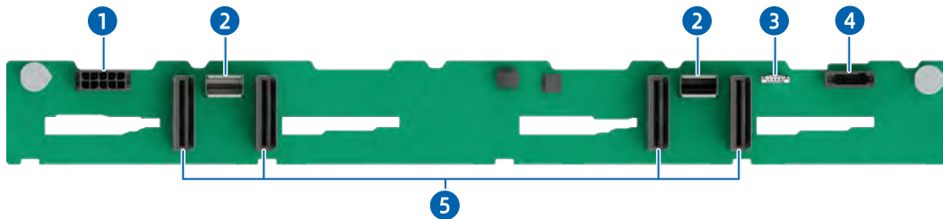
Figure 5-31 8 × 2.5-Inch SAS/SATA/NVMe Drive Backplane
