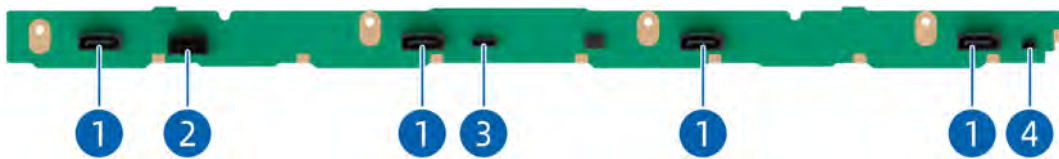
Figure 5-29 4 × 3.5-Inch SAS/SATA Drive Backplane
