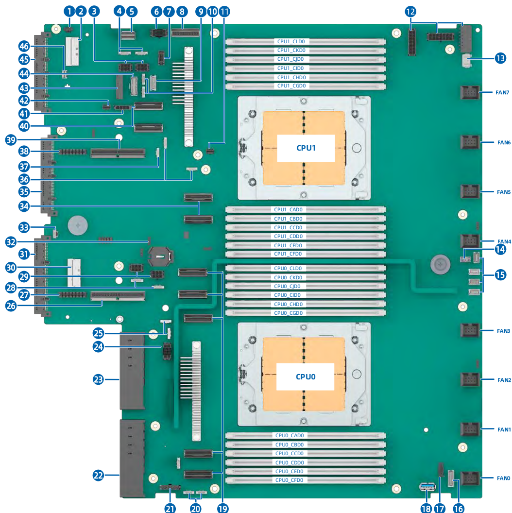
Figure 5-26 Motherboard
