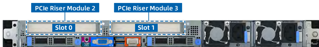
Figure 5-17 PCIe Slots
