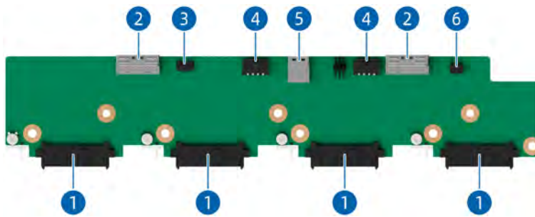
Figure 5-28 4 × 2.5-Inch SAS/SATA/NVMe Drive Backplane
