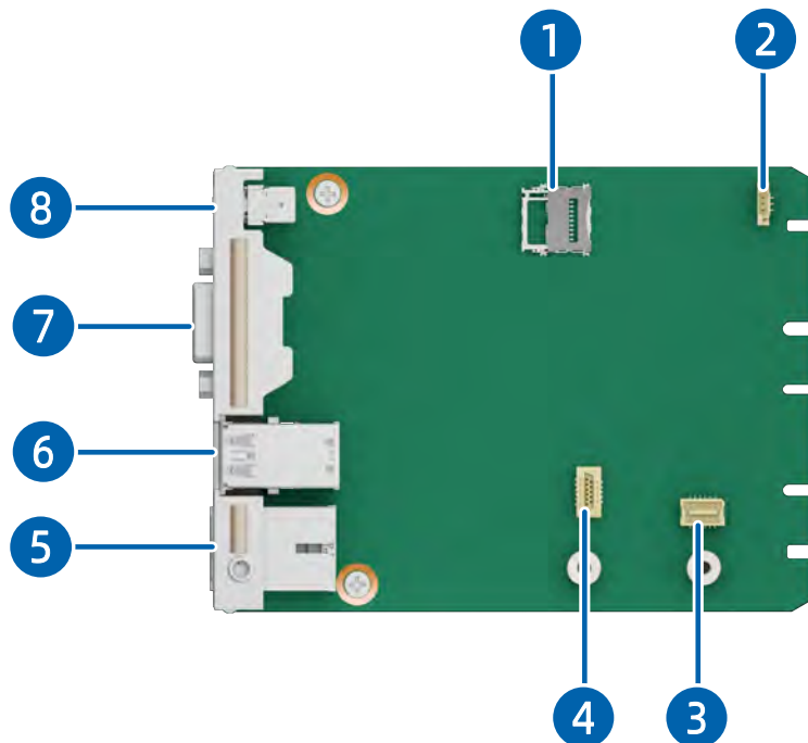
Figure 5-27 DC-SCM Board
