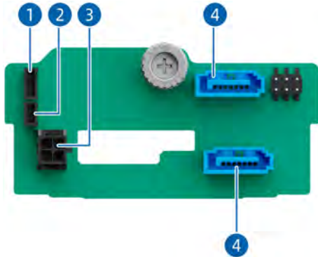
Figure 5-34 2 × 2.5-Inch SAS/SATA Drive Backplane
