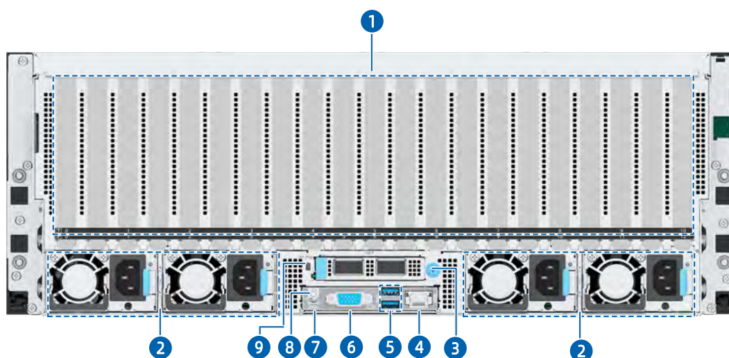
Figure 5-4 Rear View
