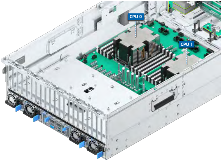
Figure 5-5 Processor Locations
