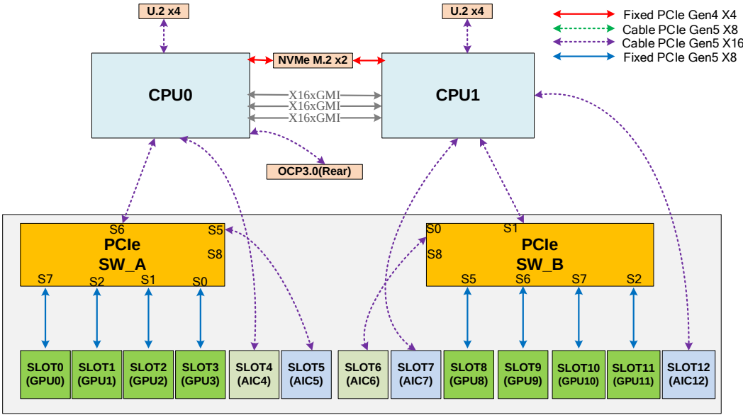
Figure 4-10 PCIe Topology Diagram for the 8 × NVMe Drive + OCP NIC Configuration
